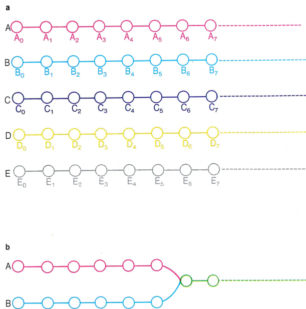
One-to-one mapping in computation. a: The left-hand end of a horizontal chain is the initial state. Motion to the right yields forward steps through a sequence of states represented by successive labeled circles. Different letters correspond to different initial states. b: When two distinguishable computational paths merge into one, information is lost. Figure 3
