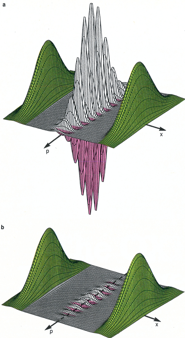
Wigner distributions. a: Distribution corresponding to the pure state of figure 3. Note the two separate positive peaks (green) as well as the oscillating interference term in between them. W(x, p) cannot be regarded as a classical distribution in the phase space as long as it has negative (red) contributions. b: Decoherence results in diffusion of W(x, p) in the direction of momentum. As a result, the negative and positive ripples of the interference term diffuse into each other and cancel out. This process is almost instantaneous for open, macroscopic systems. In the appropriate limit both the classical structure of the phase space and classical dynamics emerge naturally. Figure 5
