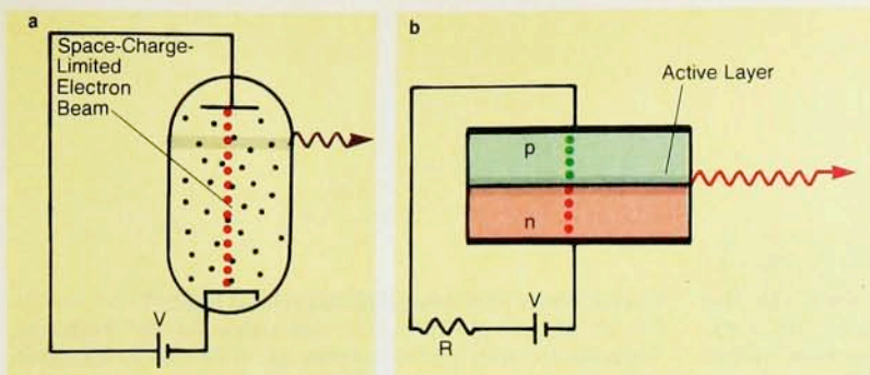
Photon-number-squeezed light can be generated by means of excitation control using both of the devices shown below. a: The Franck-Hertz apparatus contains mercury vapor (black dots). In the shaded region the electrons (red dots) have attained sufficient kinetic energy to excite the mercury atoms by means of inelastic collisions. Because of space charge associated with Coulomb repulsion, the electrons have a sub-Poisson distribution, and so too do the 253.7-nm photons (violet) emitted when the atoms relax back to the ground state. b: A similar scheme in an InGaAsP/InP distributed-feedback semiconductor injection laser. By virtue of the external resistor in series with the battery, the current flowing through the device is constant, that is, the pump fluctuations are suppressed, so that the electrons (red dots) and holes (green dots) have sub-Poisson distributions. Their recombination in the active region (shaded) generates 1.56- \mu\text{m} photons (red) with a sub-Poisson distribution. The optical feedback inherent in the laser structure enhances the effect. Figure 5
