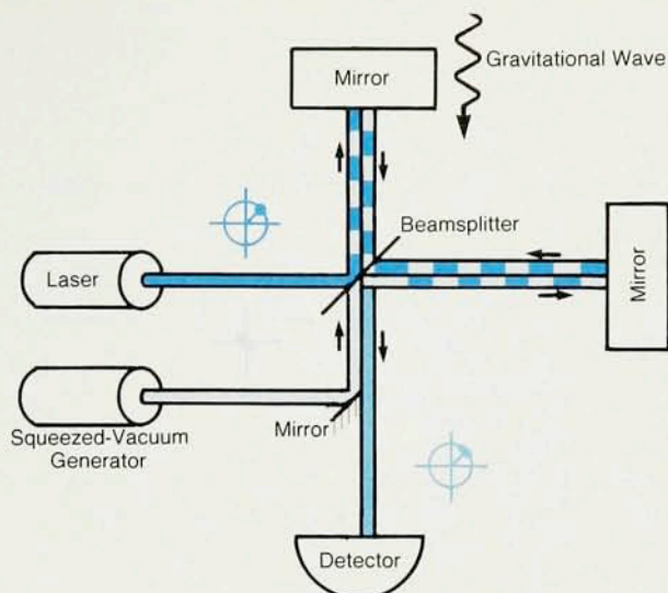
Detecting gravity waves with a Michelson interferometer. Squeezed-vacuum light entering the output port reduces the noise and improves the sensitivity, as shown by the phase-space-uncertainty sketches. Superposed beams between the arms are schematically illustrated by alternating shades of blue. Figure 7
