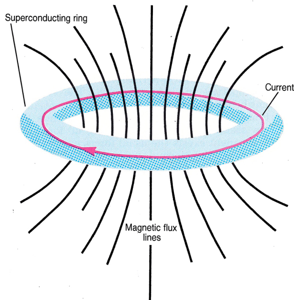
Quantized flux. The total flux threading a superconducting ring is an integral multiple of a small flux unit, \Phi_0 = hc/2e = 2 \times 10^{-7} gauss cm 2 . Figure 2
