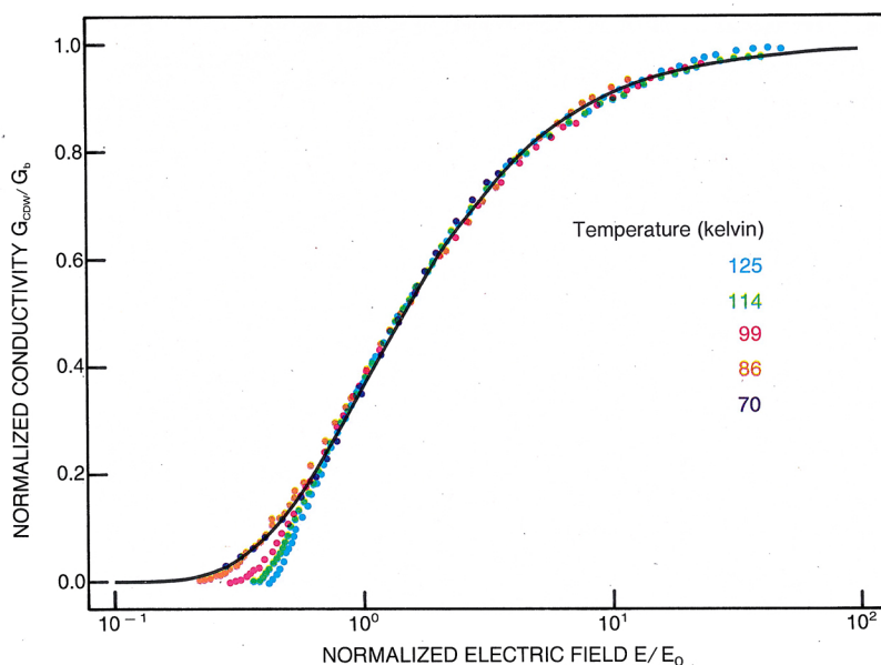
Transport in NbSe 3 . The dc conductivity, defined by G_{CDW} = I_{CDW}/E , is approximately G_b \exp(-E_0/E) . The black curve is the Zener factor, \exp(-E_0/E) . (Adapted from the PhD thesis of R. E. Thorne, "Charge-Density-Wave Transport in Quasi-One-Dimensional Conductors," University of Illinois, Urbana-Champaign, 1987.) Figure 7
