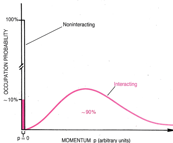
Momentum distributions of atoms in the ground state of superfluid helium-4 at T = 0 K. In a noninteracting Bose gas (shown in black), 100% of the particles are in the zero momentum state. In an interacting system (shown in magenta), because of zero-point motion the occupation probability is reduced to about 10%, but it is still finite. The probability remains finite up to the \lambda -transition temperature. Figure 1
