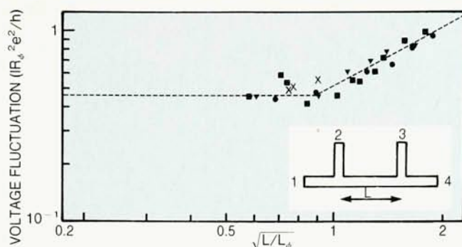
Length dependence of voltage fluctuation amplitude. Inset is a schematic of a four-lead sample. Length L between the voltage probes (2 and 3) is scaled to L_\phi , the coherence length, and voltage is normalized to IR_\phi^2 e^2/h , where R_\phi is the resistance of a length L_\phi and I is the current. Figure 5
