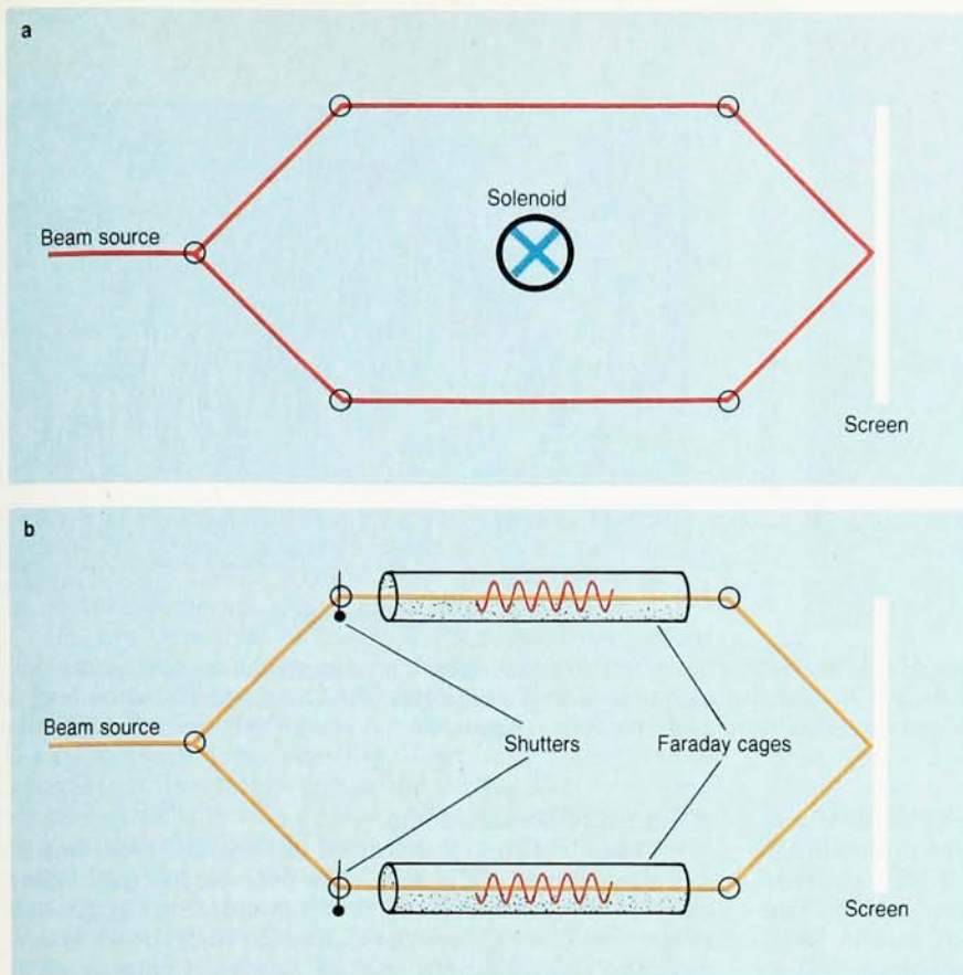
Aharonov-Bohm magnetic (a) and electrostatic (b) effects are counterintuitive consequences of quantum theory. An electron beam, split into two alternative paths, can exhibit interference effects when the beams recombine. Surprisingly, the relative phase between the two paths depends on potentials whose derivative force fields are completely shielded from the electrons. In a the phase difference is determined by the magnetic flux \Phi through a long solenoid threaded between the paths. Changing \Phi alters the interference pattern at the screen. In b the two paths are subjected to different electrostatic potentials, but only while the chopped beams are shielded within Faraday cages. Nonetheless, the potentials effect the interference. Figure 1
