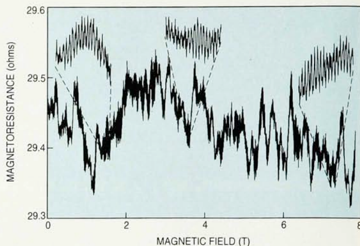
Electrical resistance of a tiny gold ring (electron micrograph, left), as a function of imposed magnetic field, measured by the authors 6 at 0.06 kelvin. The fine Aharonov–Bohm oscillations (shown expanded) correspond to a flux periodicity of h/e through the area encircled by the ring. Figure 2
