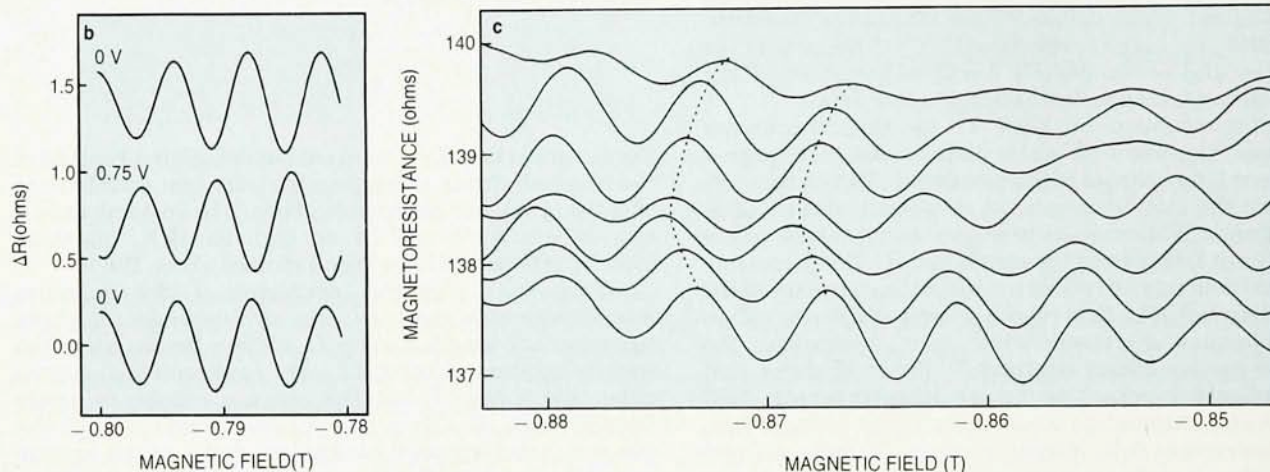
Electrostatic Aharonov-Bohm effect measured at IBM with an Sb loop 0.8 \mu\text{m} on a side, with capacitor gates along two arms. (See micrograph a.) Plot of resistance change vs magnetic field (b) shows that gate voltage (labeled) can shift oscillation phases reproducibly. Wider field sweeps (c) show gradual change of magnetoresistance pattern with increasing capacitor voltage. Each trace is measured at 0.2 volts higher than the one below. Figure 4
