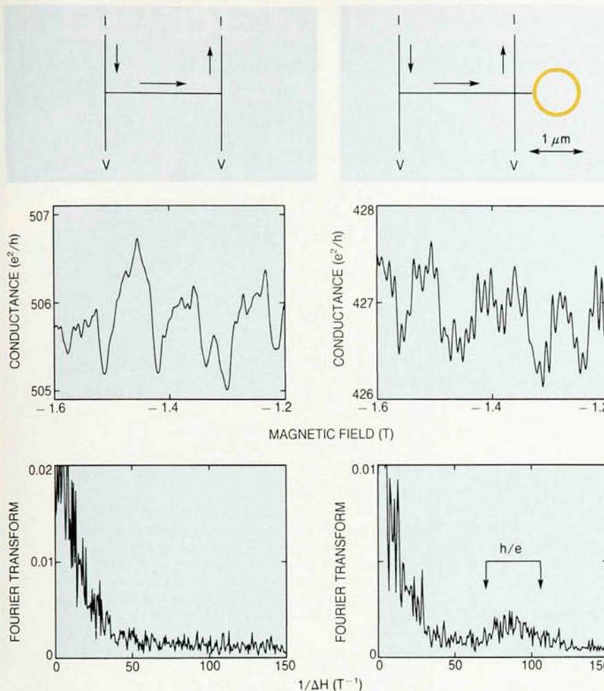
Magnetoresistance of two similar wires (schematics on top), one of which has a ring dangling outside the classical path, where it “should” have no effect. In fact the Fourier transforms of the conductance curves (bottom) show an additional peak for the circuit with the ring, indicating h/e Aharonov–Bohm oscillations corresponding to the area enclosed by the ring. Figure 7
