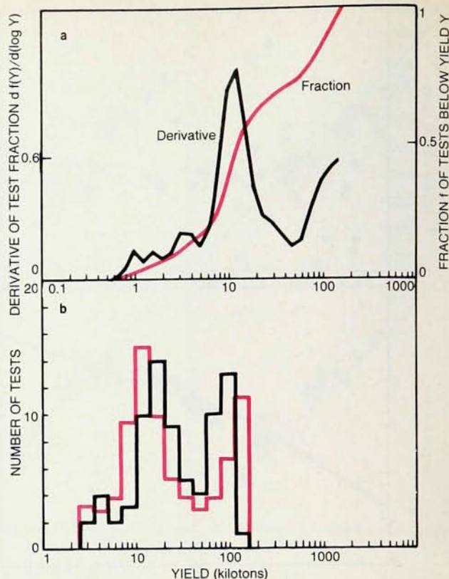
Yield distribution of explosions 4 at the Nevada test site, 1980–84. The black curve in a is the published function d f(Y)/d \log(Y) . The red curve, obtained by integration, is the implied fraction f(Y) of tests with yields at or below Y kilotons. The black curve in b is a histogram of yields calculated from announced depths when one assumes a scale depth of 450 feet for all explosions. The red curve in b is a histogram based on the red curve in a. This histogram and those in subsequent figures are terminated at 2.5 kilotons with yield-bin boundaries increasing by a factor of 2^{1/2} . Figure 5
