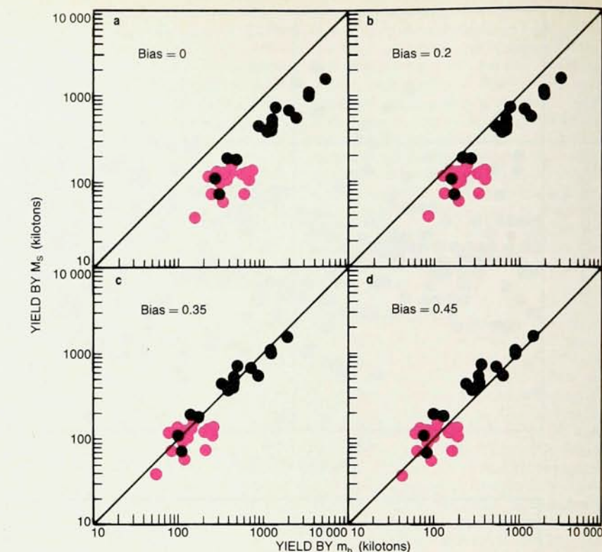
Calculated yields for 33 Soviet tests with accurately determined seismic magnitudes m_b . The yield of each test was calculated two different ways—by its seismic magnitude m_b and by its seismic magnitude M_S . The two methods give the same results when one assumes a bias to correct for seismological differences between US and Soviet test sites. Black points represent tests at Novaya Zemlya; red points, tests at Semipalatinsk. 4 Figure 3
