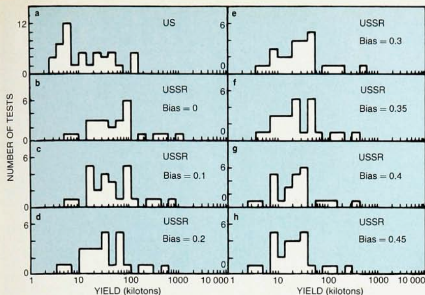
Histograms of yields for the US and Soviet test programs during the first three years of underground tests. Yields for US tests during 1963-65 were calculated using announced depths and a scale depth of 450 feet. Yields for Soviet tests during 1964-66 were calculated using National Earthquake Information Service magnitude values, equation 2 and the indicated biases in the magnitudes m_b .
