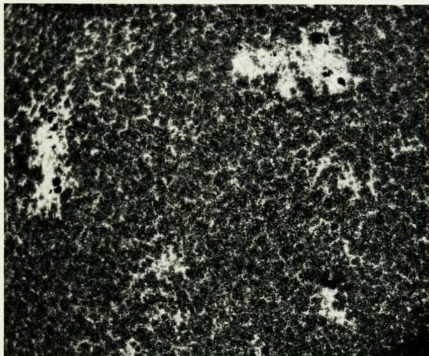
Portion of the Sun in a 100-Å band centered at 1600 Å. Sunspots and active regions are readily recognized in this photo, as is the network pattern associated with the edges of the supergranular convective cells. Note the numerous bright dots within the cells. The photo clearly illustrates the highly structured nature of the Sun's atmosphere. (The figure is reprinted by permission of the publisher from Physics of the Sun .)
