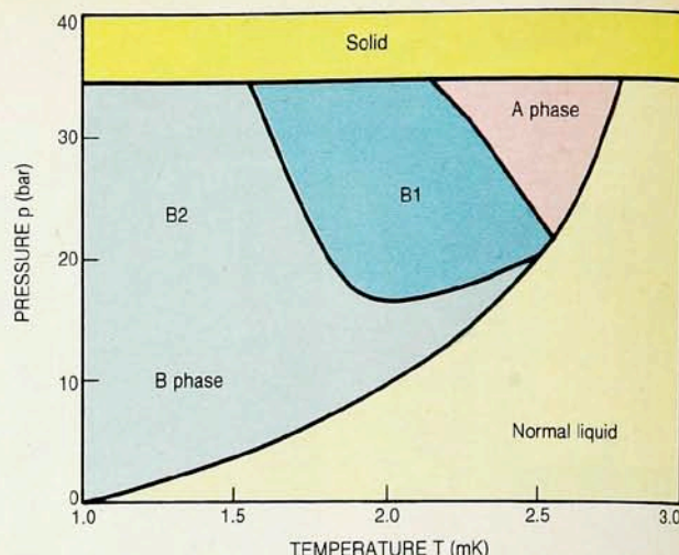
Phase diagram of He 3 below 3 mK. There are two superfluid phases, A and B, and the rotating B phase exhibits a phase transition between two vortex structures, B1 and B2. At a pressure of 21.2 bar and a temperature of 2.55 mK the three liquid phases are in thermal equilibrium with one another. To convert the temperatures given in this article to those of the most recent scale, proposed by Dennis Greywall, multiply our figures by 0.89. Figure 2
