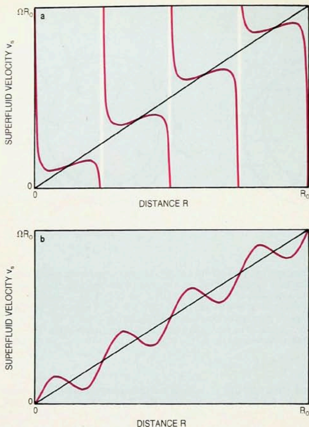
Tangential component of the superfluid velocity field v_s as a function of distance from the center of a rotating cylinder. a: Singular vorticity. b: Continuous vorticity. The diagonal lines indicate the relationship for a solid body rotating with angular velocity \Omega .
