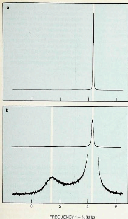
Transverse nmr absorption in He 3 -A at a temperature of 0.73 T c and pressure of 29.3 bar in an axial magnetic field of 28.4 mT. The graphs show the absorption as functions of frequency when the cryostat is at rest (a) and when it is rotating at \Omega = 1.21 rad/sec (b). The lower graph in b shows a vertically expanded view of the satellite peak. 3
