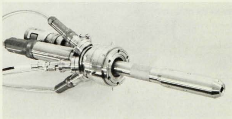
EMG-12 20 keV RHEED GUN ON 70 mm (2 3 / 4 in.) CONFLAT
