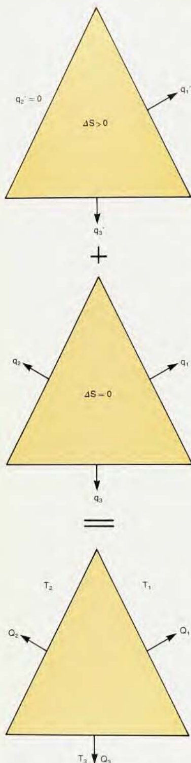
Tricycle engine. A simple general engine (bottom) operates at three different temperatures T_1 , T_2 , T_3 , absorbing or releasing heat at each temperature. Work is simply heat transferred at infinite temperature (that is, zero entropy). Such a cycle can always be decomposed as shown into a reversible part (middle) and an irreversible flow of heat from T_1 to T_3 (top).
