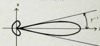
Laboratory frame
