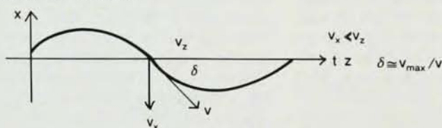
Laboratory frame
