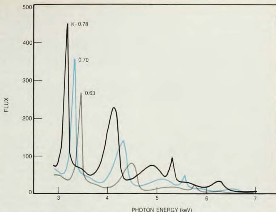
Higher-harmonic spectrum produced by 3-GeV electrons in the LBL-SSRL 30-period permanent-magnet undulator. Slits were used to define a very small angular acceptance ( 18 \times 10^{-6} radians horizontal, 8.8 \times 10^{-6} radians vertical.) Figure 9.
