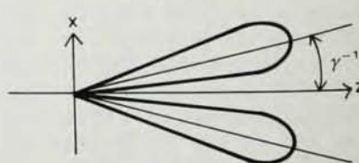
Laboratory frame
