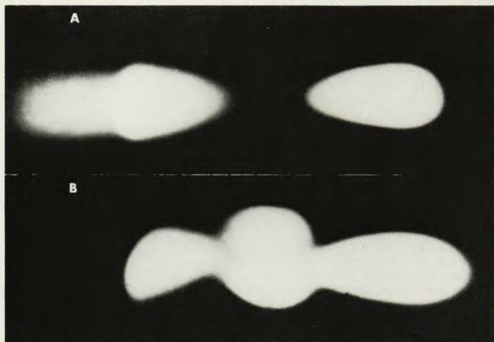
First observation of undulator radiation (reference 6) from a circular electron machine—the Pachra 1.3-GeV synchrotron at the Lebedev Physics Institute, Moscow. (a) Undulator off : The two lobes are synchrotron radiation from the bending magnets adjacent to the undulator. (b) Undulator on : The central spot is due to the undulator. The electron energy is 175 MeV. (Courtesy V. V. Mikhailin, Moscow State U.)
