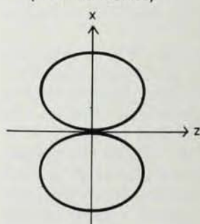
Rest frame
