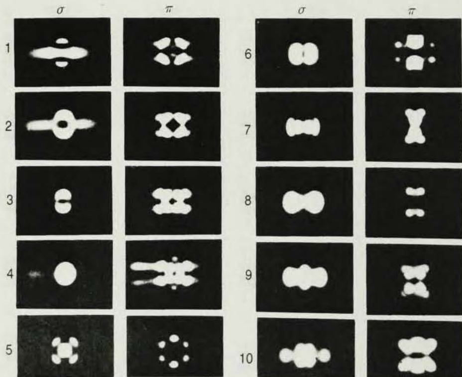
Undulator radiation patterns for different polarization and varied electron energy. The angular distribution is shown at a wavelength of 500 nm with polarization parallel ( \sigma ) and perpendicular ( \pi ) to the electron acceleration vector at electron energies ranging from 473 MeV (1 \sigma, \pi ) to 97.5 MeV (10 \sigma, \pi ). The undulator had a period of 14 cm and was operated at 0.839 kG. (Reference 7)
