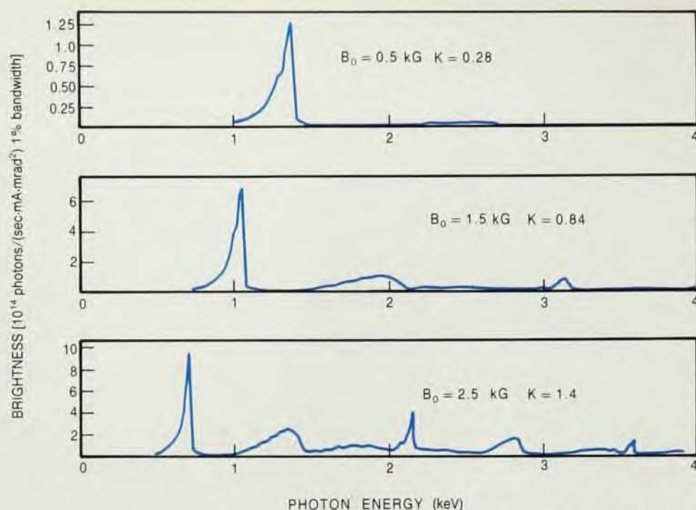
Spectra from undulator magnet at LBL-SSRL calculated for 3.0 GeV and different values of the peak magnetic field. The effects of finite electron beam size and divergence have been included. The detector is assumed to be 25 m away from the undulator. (Program Sy Y. Sambre, Stanford.)
