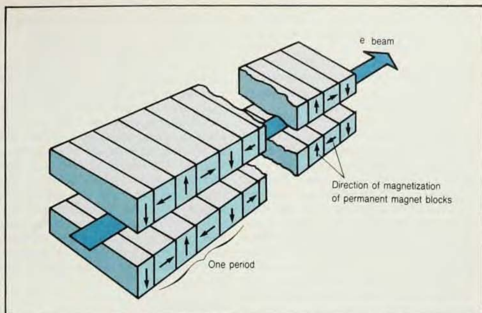
Permanent-magnet undulator with vertical field made from blocks of rare-earth-cobalt ( \text{SmCo}_5 ) material. The beam is shown traveling in a straight line because the amplitude of oscillation is very small (typically 0.02 nm) compared to the beam width. Figure 8.
