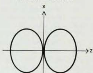
Radiation Patterns
