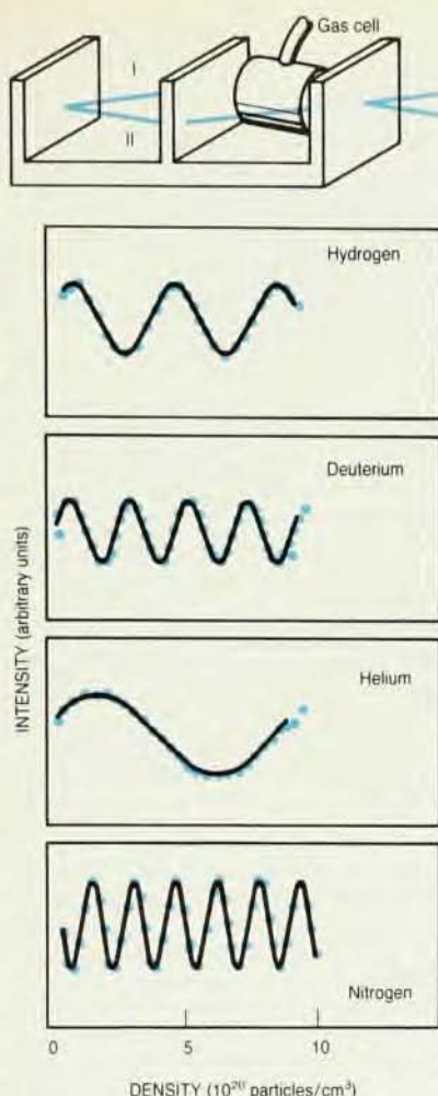
Interference oscillations for various gases. As the diagram at top shows, a gas cell introduces a phase difference between paths I and II. The rate at which the phase changes with density serves to measure the scattering length of the gas. Figure 3
