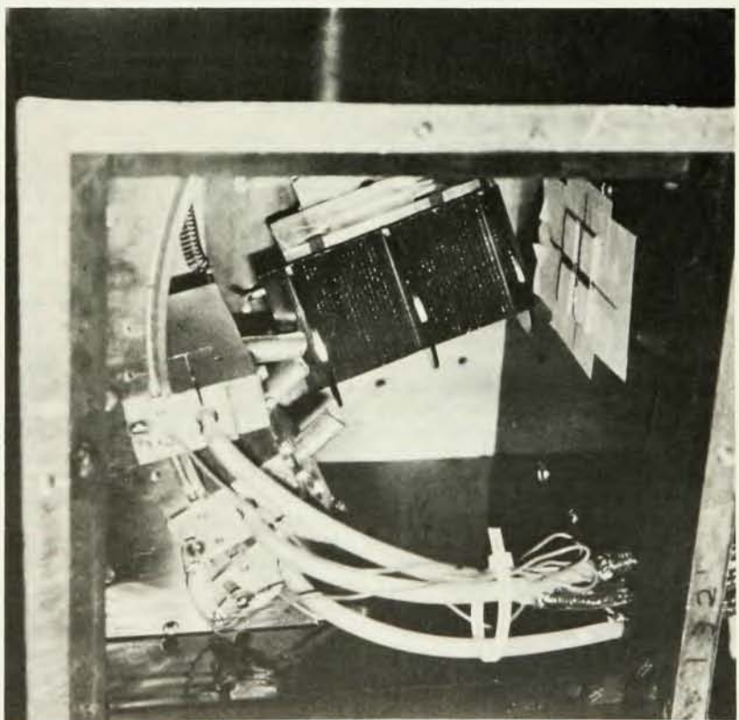
The neutron interferometer used in the author's laboratory at the University of Missouri. The upper photo shows the silicon slabs machined from a single crystal of high-purity silicon to maintain alignment of the crystal planes from slab to slab. The lower photo shows such an interferometer in place in its housing at the reactor. The entrance slit is at the left and the three counters C_1 , C_2 and C_3 (see figure 2) are on the right.
