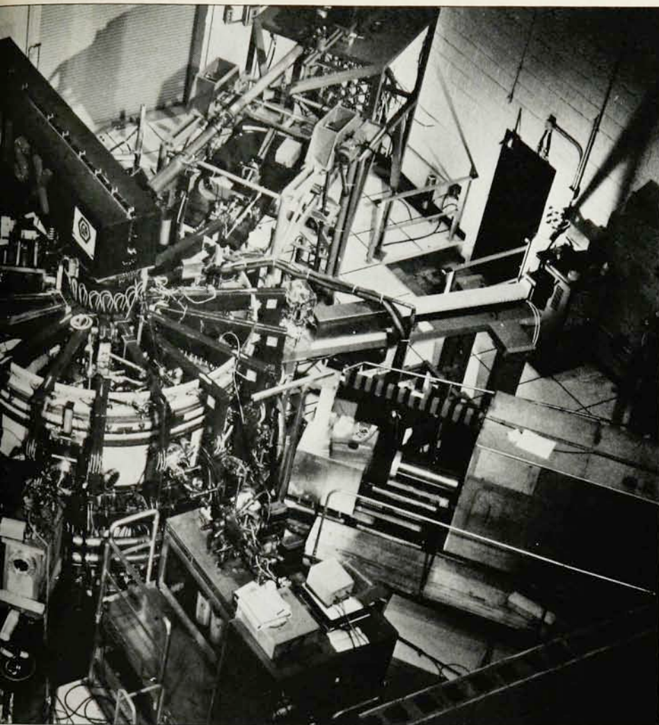
The ISX tokamak at Oak Ridge National Laboratory. It is surrounded by beam injectors and diagnostic apparatus. The toroidal vacuum chamber is within the current-carrying coils. The large iron yoke serves as the core of a transformer whose secondary is the plasma itself; the induced currents heat the plasma. Tokamak devices are among those that may be suitable for hybrid fusion-fission reactors. (Photo courtesy of ORNL)
