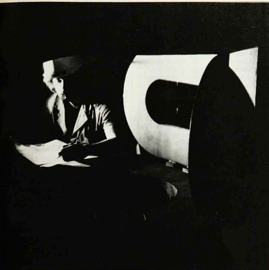
The tandem mirror machine at Lawrence Livermore Laboratories. On the left is the interior of the central tube. A technician is tightening down the titanium "getter" wires; after each plasma pulse titanium is evaporated from these wires and deposited on the vacuum-chamber walls to cover adsorbed impurities. The large coils provide a focussing field for the plasma beam. It is this part of the machine that could be surrounded by a blanket of fertile material to produce fissile isotopes for use in ordinary fission power plants. On the right is a "beam's eye view" of one of the two magnetic mirrors that are at the ends of the tube shown at left. Note that the main coil for the mirror is shaped like the seam of a baseball. (Both photos by David Proffitt, Lawrence Livermore.)
