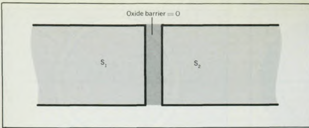
Two superconductors S_1 and S_2 separated by an oxide barrier O . Ivar Giaever's experiments in 1960 demonstrated the tunneling of electrons through a 20-30 Å oxide layer. Figure 4
