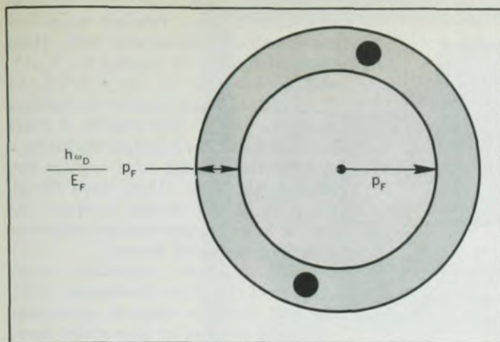
Two electrons interacting via an attractive potential -V above a quiescent Fermi sea; p_F is the Fermi momentum. Figure 2
