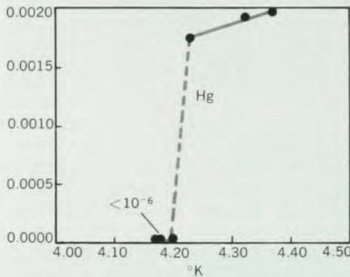
Kamerlingh Onnes's data on the superconductivity of mercury. Figure 1
