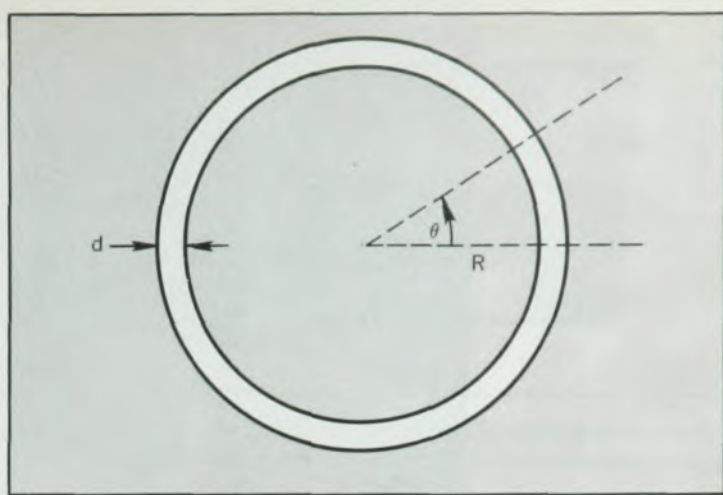
In a circular loop of superconducting wire the superfluid wavefunction is coherent over macroscopic distances. Figure 3
