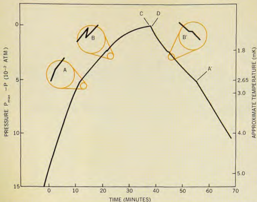
Pressurization curve for \text{He}^3 shows a sudden change in slope at 33.9 atm and 2.65 mK that is highly reproducible during both compression (A) and decompression (A'). Second slope change (B, B') is complicated by hysteresis during the compressive part of the cycle, which may be caused by supercooling. The behavior of this system does not appear to agree with a simple antiferromagnetic phase transition.
