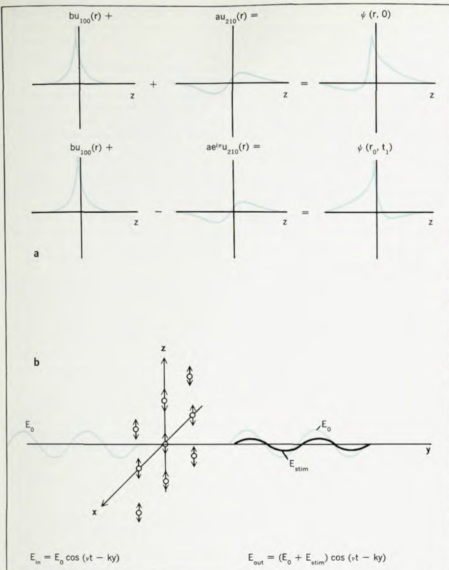
Radiating dipoles. The z -dependence of the wave function \psi(r,t) in part (a) are for t = 0 and t = \pi/\omega ; the probability density \psi^*\psi oscillates back and forth across the nucleus at frequency \omega , so yielding an oscillating dipole. Part (b) of the figure shows how a sheet of dipoles radiates an electric field in phase with the incident field (equation 2). The individual fields become increasingly retarded the further off the axis one goes. Figure 2
