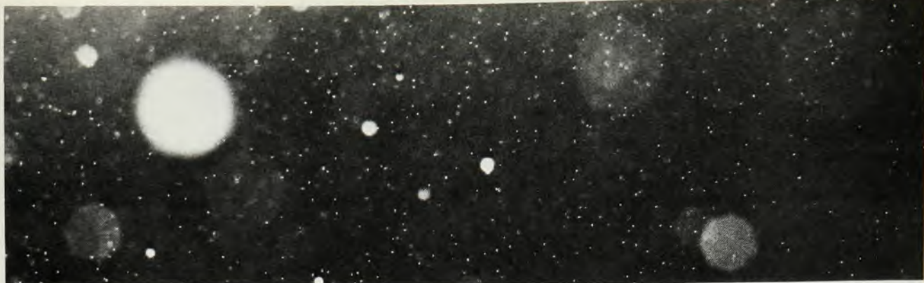
Cloud droplets and ice particles in cumulus cloud, 15 June 1972, near Sterling, Colorado. The altitude was 7 km and the temperature -14^{\circ}\text{C} . Ice-particle diameters are in the range 0.5–0.8 mm, and their concentration is approximately 200 per liter. Cloud droplet concentration is greater than 91\text{ cm}^{-3} ; radii are not more than 100 microns. Figure 6
