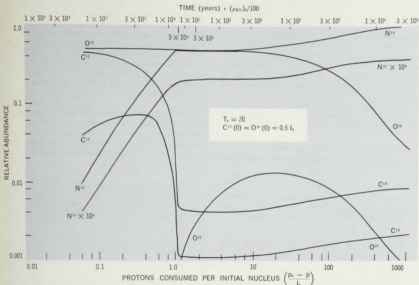
VARIATION WITH TIME of the abundances of various elements involved in the CNO cycle. It is assumed that initially C^{12} and O^{16} have the same abundance while that of N^{14} is small. From G. R. Caughlan, Astrophys. J. (1967). —FIG. 5
