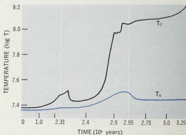
EVOLUTION OF A STAR of 3 solar masses, according to I. Iben, Astrophys. J. 142, 1447 (1965). Abscissa is time in units of 10^8 years (note the breaks in scale at t = 2.31 and 2.55 ). I. Temperature (on logarithmic scale): T_c = temperature at center of star, T_s = same at midpoint of source of energy generation, which after t = 2.48 is a thin shell. T_c increases enormously, T_s stays almost constant.
