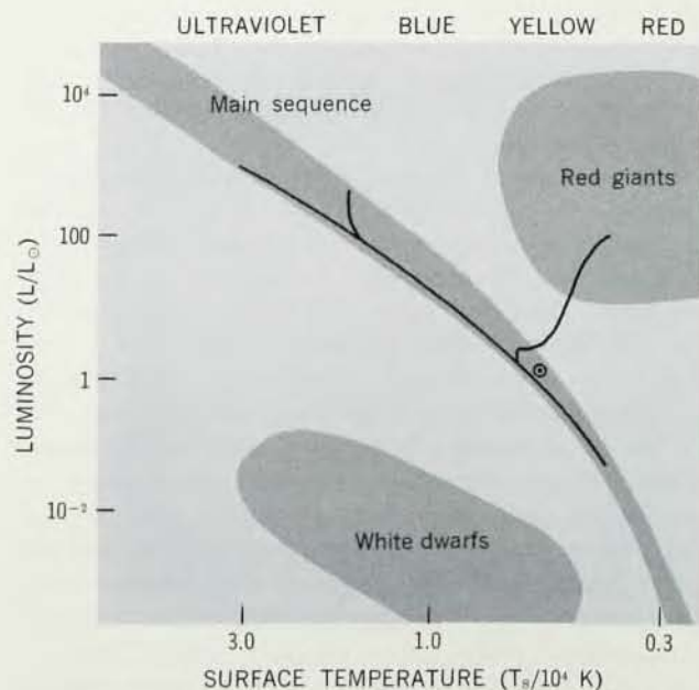
HERTZSPRUNG-RUSSELL DIAGRAM. From E. E. Salpeter, in Apollo and the Universe , Science Foundation for Physics, University of Sydney, Australia (1967). —FIG. 1
