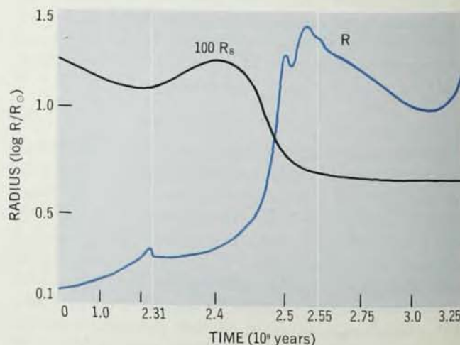
EVOLUTION OF A STAR, see caption to figure 6. II. Radius, in units of that of the sun, on logarithmic scale. R = total radius, 100 R_s = 100 times the radius of midpoint of energy source. R increases tremendously, while R_s shrinks somewhat.
