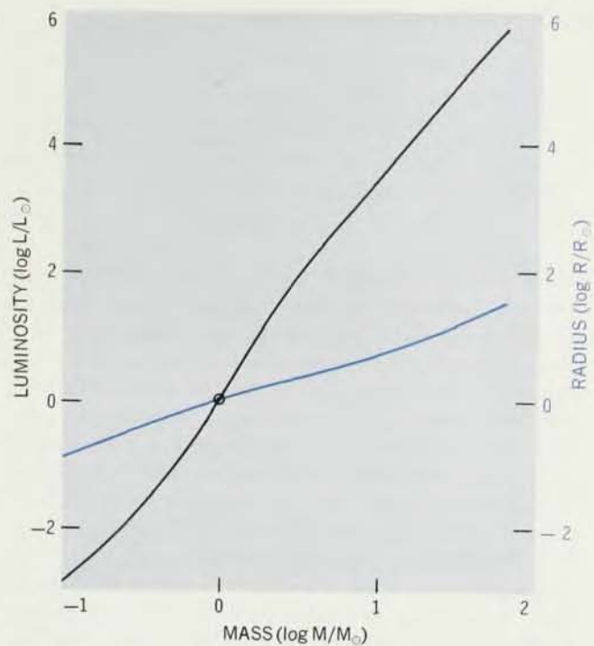
LUMINOSITY AND RADIUS of stars vs mass. Abscissa is \log M/M_\odot . Data from C. W. Allen, Astrophysical Quantities (Athlone Press, 1963), p. 203. The curve for \log L/L_\odot holds for all stars, that for R/R_\odot only for the stars in the main sequence. The symbol \odot refers to the sun. —FIG. 2
