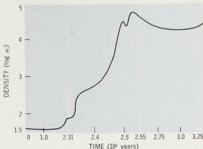
EVOLUTION OF A STAR, see caption to figure 6. III. Density, on logarithmic scale, at the center of the star. This quantity increases about 1000-fold. —FIG. 8
