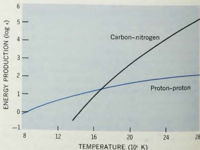
THE ENERGY PRODUCTION, in erg/gm sec, as a function of the temperature in millions of degrees, for the proton-proton reaction (P P) and the carbon-nitrogen cycle (C N). Concentrations assumed X = Y = 0.5 , Z = 0.02 . Calculated from Tables 8 and 9 of Reeves, reference 12. —FIG. 4
