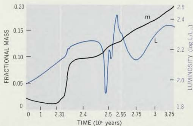
EVOLUTION OF A STAR, see caption to figure 6. IV. Curve L , luminosity relative to that of the sun, on logarithmic scale. This quantity does not change very much during the life of the star. Curve m , fraction of the mass of the star enclosed by energy-producing shell, on linear scale. This fraction increases slowly with time. —FIG. 9
