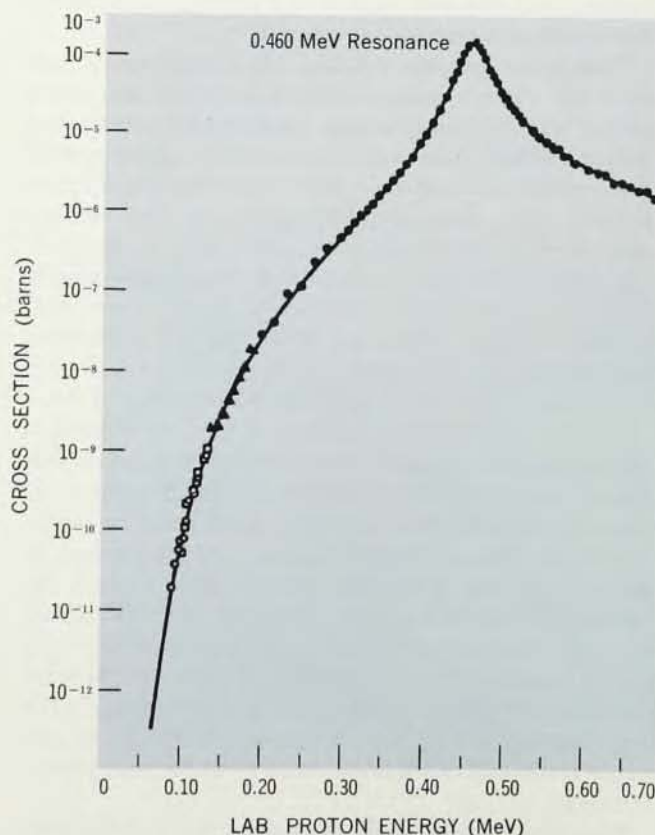
CROSS SECTION for the reaction \text{C}^{12} + \text{H} , as a function of the proton energy. From Fowler, Caughlan and Zimmerman, reference 5. —FIG. 3
