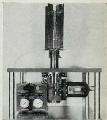
ADL-Collins Helium Liquefier. For 20 years the standard for low-temperature research installations, this semiautomatic machine is available in 25, 50, 100, and 200-liter-per-day capacities. Refrigerator models: 200 watts at 20°K and 30 watts at 4.2°K. Two models for hydrogen/helium liquefaction.
