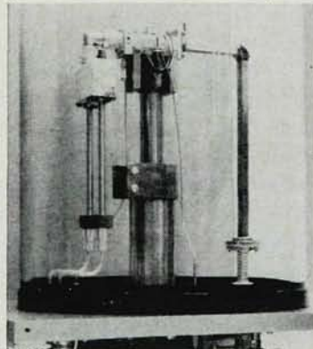
ADL CRYODYNE® Parametric Amplifier Refrigerator. A standard in the microwave field for cooling low-noise amplifiers in fixed or mobile systems, this 20°K machine can be operated continuously for 3,000 hours before preventive maintenance is required.
