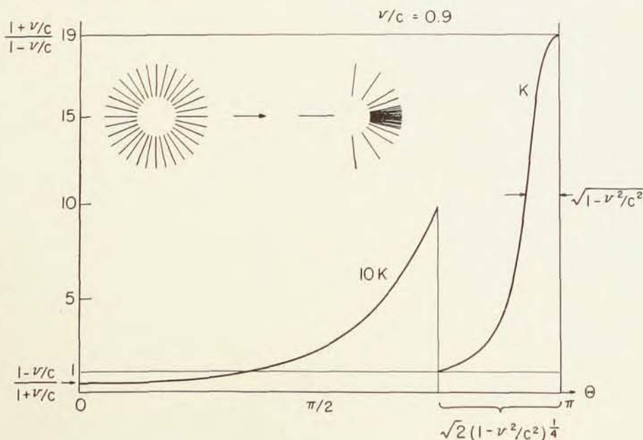
Fig. 5. The ratio K of the emitted intensity per solid angle measured in the observer's system to the intensity per solid angle measured in the system moving with the object, as function of the angle \theta of observation. K also determines the Doppler shift. The observed frequency \omega is related to the emitted frequency by \omega = K^{1/2}\omega_0 .
