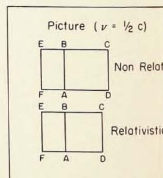
Fig. 1. A cube moving with velocity v seen by an observer at an angle of 90^\circ .
