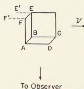
Fig. 1. A cube moving with velocity v seen by an observer at an angle of 90^\circ .
