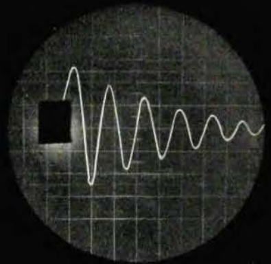
Oscillograph from which resonant frequency, Q, and voltage reversal can be determined.
