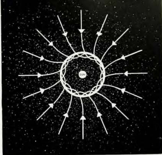
The charged atoms spiral inward to form rings of gas (only one is shown here) which might later condense into planets.
