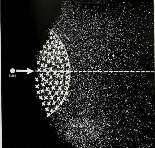
The sun, rushing through space at twelve miles per second, passes through a gaseous nebula. Its presence creates electric charges on the atoms of gas.
