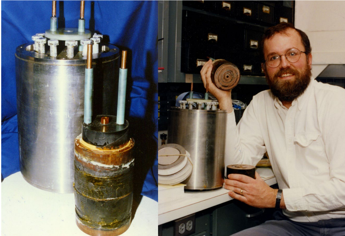
Figure 2: The two world-record 72T pulsed magnets. [18] At left is the completely assembled magnet, housed in the VascoMax steel casing used to precompress the magnet coil... and to contain any “magnet disassembly events.” At right is the magnet coil removed from its casing, wound with three different conductors chosen for high ductility (layer 1), high strength (layers 2-7), and high conductivity (layers 8-14). Figure 3: One of world-record 72T pulsed magnets [18], shown with the author holding two halves of a second magnet coil (cut in half to facilitate post-pulse analysis). The experimental sample and plastic cryostat tails fit inside the 9.2mm diameter clear bore of the magnet coil at the center of the coil windings. At extreme left is one of the twelve thyristors used to switch the capacitor bank that energized the magnets. The thyristors were stacked three in series and four in parallel to handle the 12kV voltage and 325kA current specifications, respectively.
